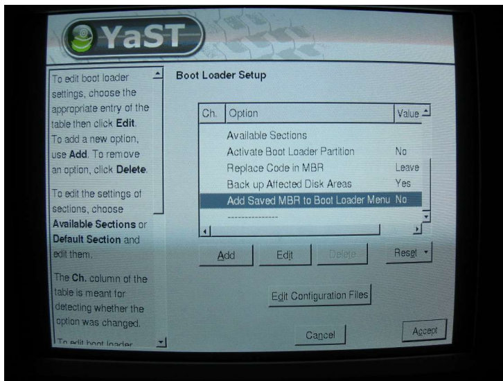
Figure 9. After modifying the Replace Code in MBR option, the result is shown in the Boot Loader Setup screen.
