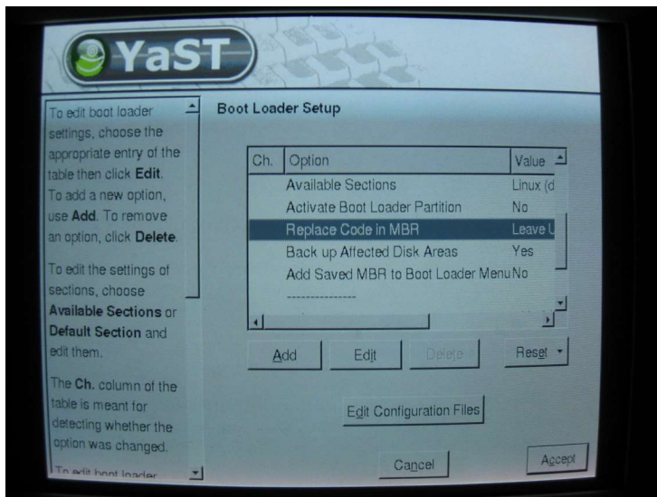
Figure 7. Editing boot loader options in SuSE.
