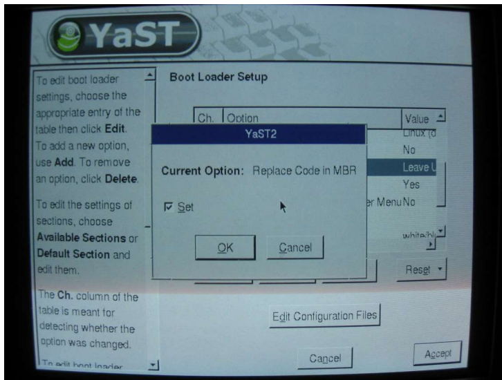
Figure 8. The Replace Code in MBR dialog.
